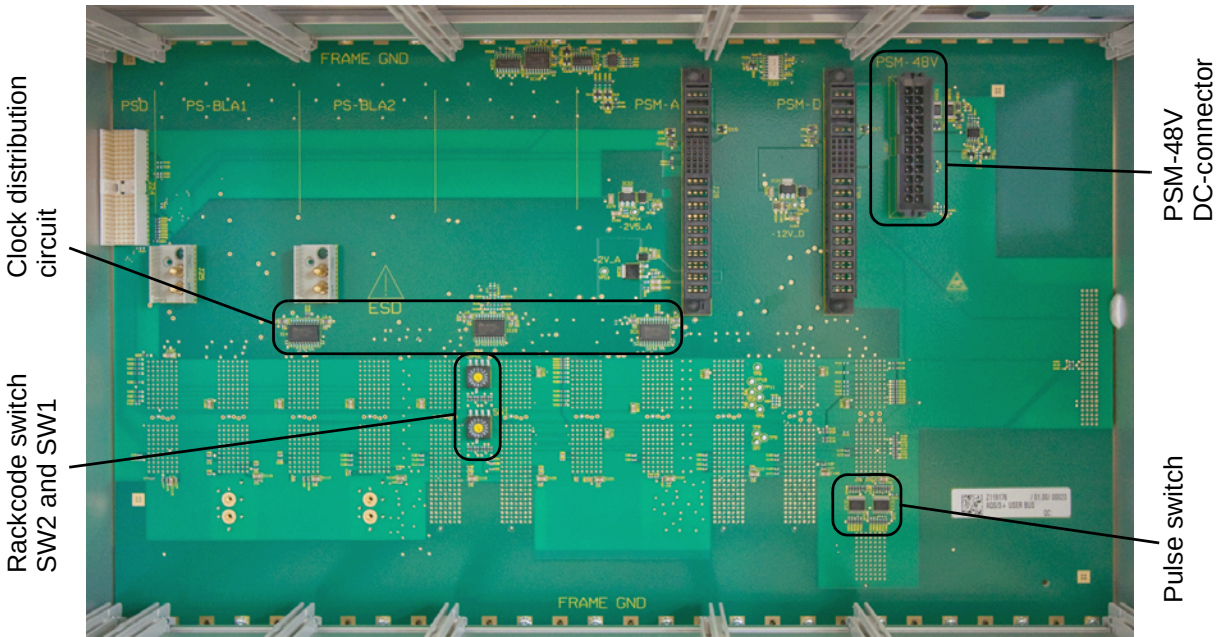
Figure 7.6 AQS/3+ User Bus (front view)
