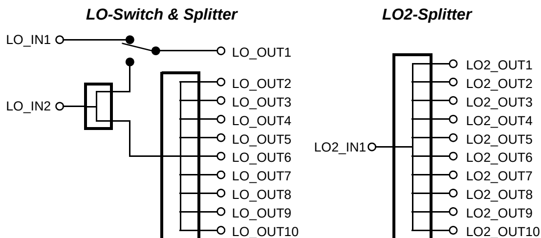
Figure 14.2 LO/LO2- Splitter
